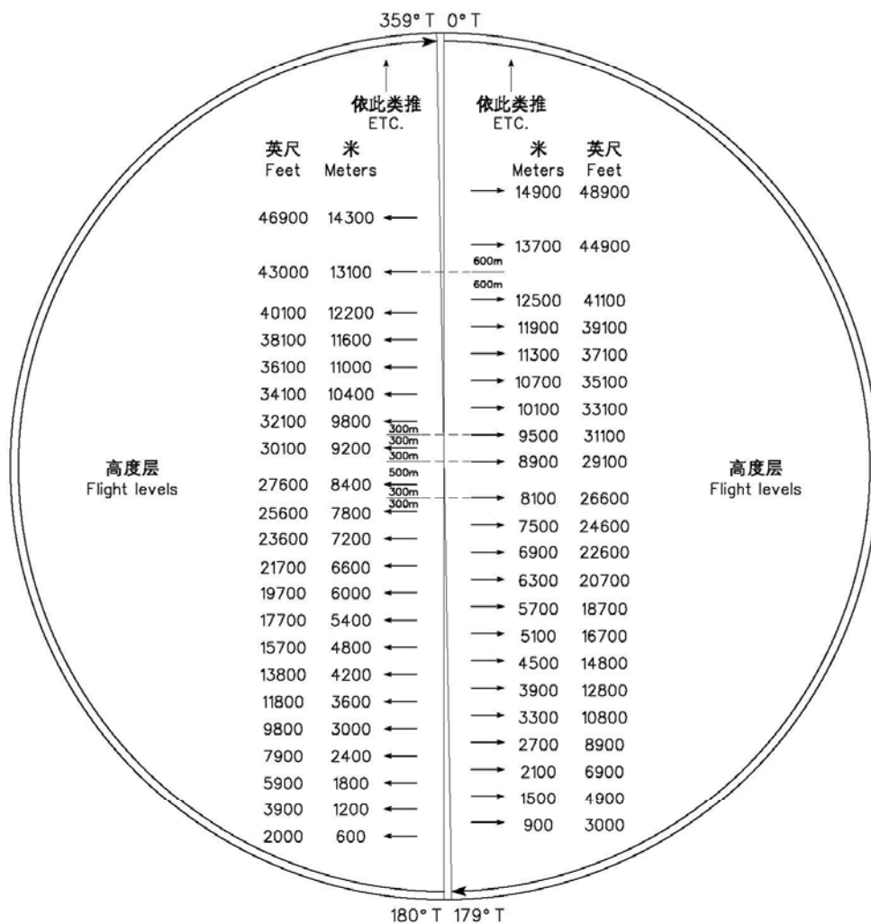
飞行高度层配备示意图 Diagram of Flight Levels Allocation
